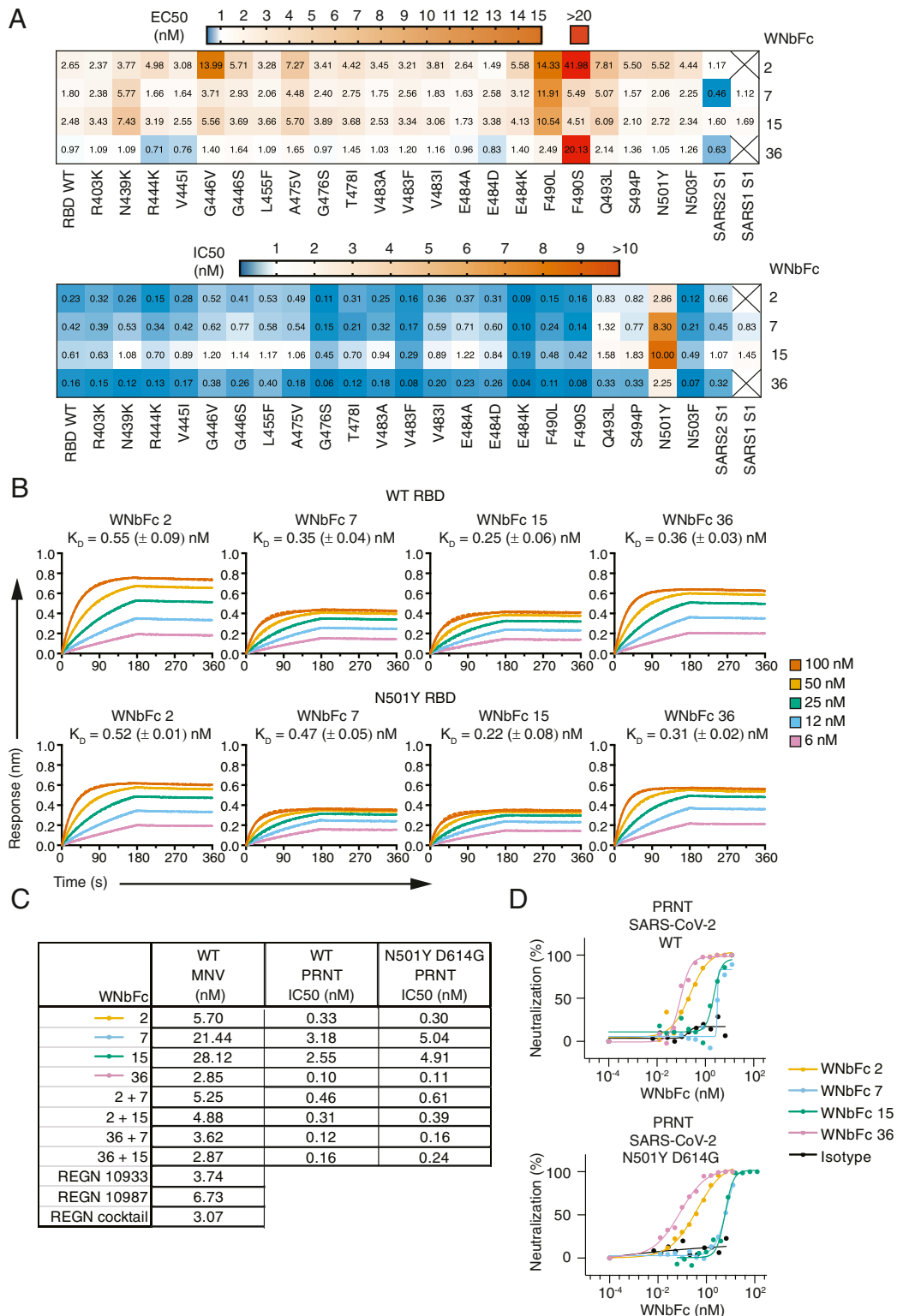
Fig. 2. Antibody affinities and neutralization potencies of bivalent nanobody-Fc fusions. (A) Heatmap of WNbFc nanobodies binding to RBD variants with the range of relative EC_{50} shown [nanomolar (nM)] (Top) and blocking of ACE2 interaction with the range of relative IC_{50} shown (nM) (Bottom) using the RBD global variant multiplex arrays. Squares with crosses represent nonbinders and noninhibitory nanobodies in top and bottom, respectively. (B) Bio-layer interferometry affinity measurements with immobilized WNbFc fusion and SARS-CoV-2 RBD in solution. Representative binding curves of five different RBD concentrations from 6 to 100 nM to immobilized nanobodies are plotted (solid line) and were fitted to a 1:1 binding model (dashed line). Corresponding mean \pm SEM. K_D values are indicated, and representative binding curves are shown from three independent experiments. (C) Neutralization of WT or N501Y D614G SARS-CoV-2 using the MNV and PRNT assay. For MNV, the values are the geometric mean of n = 2 to 4 biological replicates. For PRNT, the value is representative of two biological replicates with duplicate technical replicates per concentration. (D) Inhibition of WT and N501Y D614G SARS-CoV-2 virus using PRNT. For PRNT, the value is representative of two biological replicates with duplicate technical replicates per concentration.
